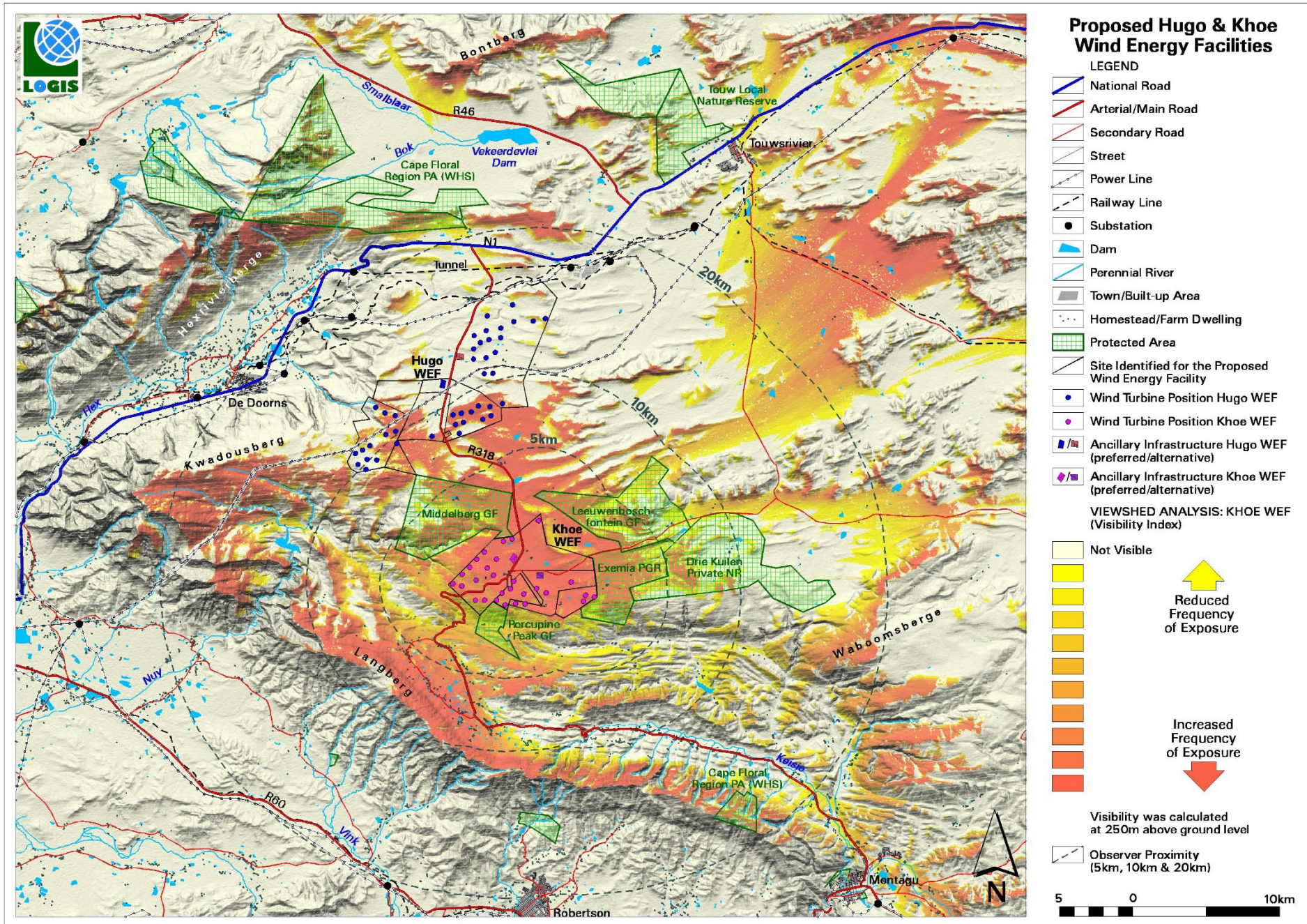
Map 3: Viewshed analysis of the proposed Khoe Wind Energy Facility, indicating the frequency of visual exposure
