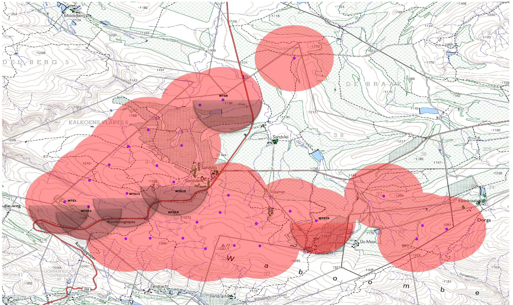
Map 9: Potential sensitive receptors exposed to shadow flicker from the proposed Khoe Wind Energy Facility
