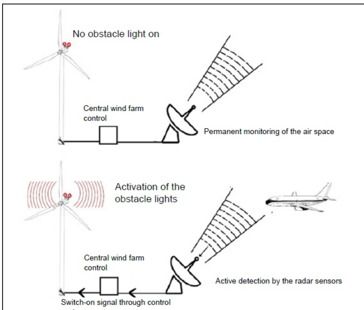
Figure 64: Diagram of the functional principle of the needs-based night lights.
